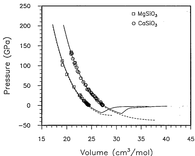
FIG. 1. Equations of state for \text{CaSiO}_3 and \text{MgSiO}_3 perovskite. Solid lines are results from the 300 K constant volume MD simulations. Dashed lines correspond to the static lattice (athermal) calculations. The experimental data for \text{CaSiO}_3 (Refs. 31 and 36) and \text{MgSiO}_3 (Refs. 34 and 35) is displayed with open symbols. The onset of amorphization are the constant volume and constant pressure MD simulations occurs at 31 \text{ cm}^3/\text{mol} for \text{CaSiO}_3 perovskite and 27 \text{ cm}^3/\text{mol} for \text{MgSiO}_3 perovskite, both occurring under tension near -18 \text{ GPa} at 300 K. At larger volumes there is a gradual buildup of lattice defects with a reduction in tension.
