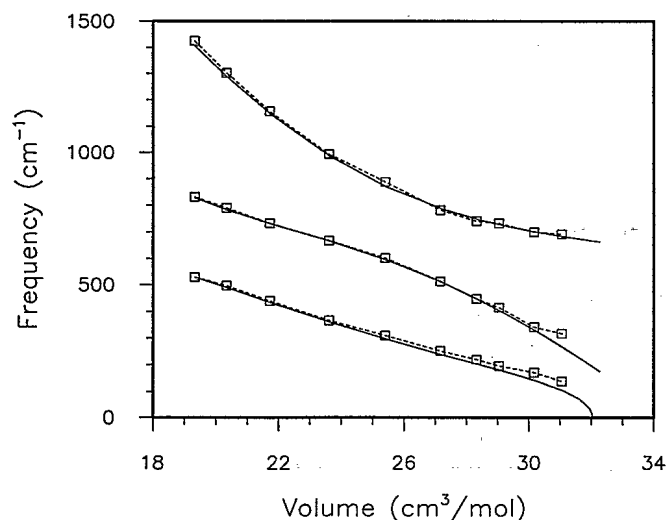
FIG. 5. Volume dependence of the transverse-optic mode frequencies ( \Gamma_{15} ) at the Brillouin-zone center of the cubic perovskite Pm\bar{3}m phase of \text{CaSiO}_3 . Solid lines are the quasiharmonic frequencies calculated from lattice dynamics and dashed lines with symbols are frequencies obtained from the MD simulations at 300 K through a Fourier transform of the electrical flux autocorrelation function.
