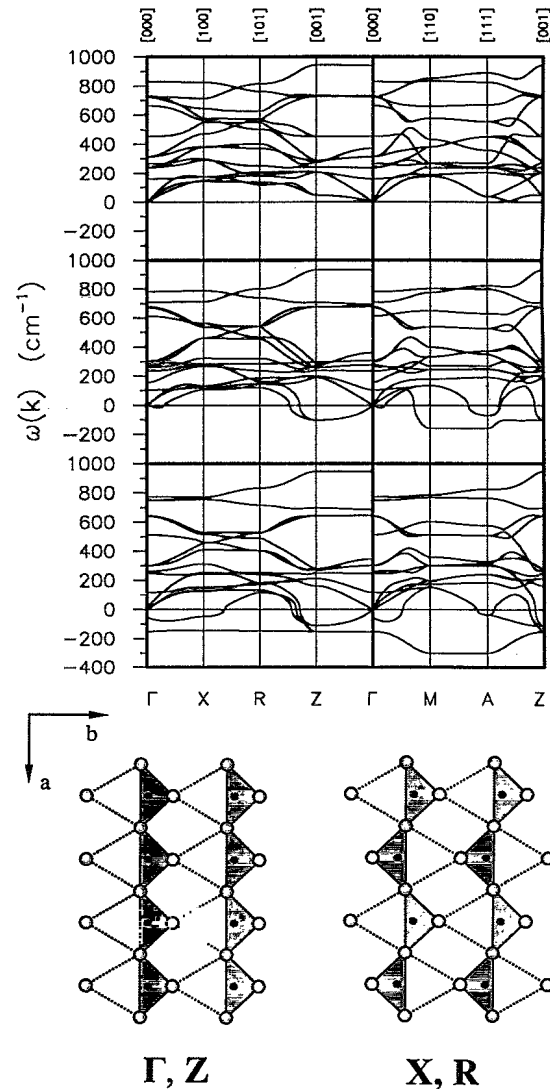
FIG. 7. (a) Quasi-harmonic phonon-dispersion relations for the \text{CaSiO}_3 P4mm phase at -12 , -18 , and -20 GPa. At -12 GPa the P4mm phase is dynamically stable. The first instability occurs at -12.5 GPa for an incommensurate mode along the Brillouin-zone boundary between A and Z at \mathbf{k}=(0.636, 0.636, 1) . At -18 GPa, entire acoustic branch in the \Gamma - M - A - Z - \Gamma plane is unstable. This branch corresponds to various rotational and deformational motions of the \text{SiO}_5 polyhedra. At -20 GPa, an entire optic branch in the \Gamma - X - R - Z - \Gamma plane also becomes unstable in the constrained P4mm structure. Condensation of any mode along this nearly dispersionless results in the transformation of the P4mm structure to a pyroxenelike structure made up of corner-linked chains of silica tetrahedra. (b) The different pyroxenelike structures which result from condensation of the unstable optic mode at the \Gamma , Z , X , and R points. Condensation of the \Gamma mode results in the formation of parallel chains of corner-shared \text{SiO}_4 tetrahedra where each tetrahedra has the same spatial orientation. Condensation at the Z point results in a structure similar to that obtained from \Gamma except that adjacent chains above and below the a - b plane (not shown in the figure) have an opposite orientation. Condensation of the X mode results in the formation of tetrahedral chains with a two-unit repeat in the x direction. Condensation at R results in a similar structure to that obtained from X except that the orientation of the tetrahedra is opposite in adjacent chains above and below (not shown) the a - b plane.
