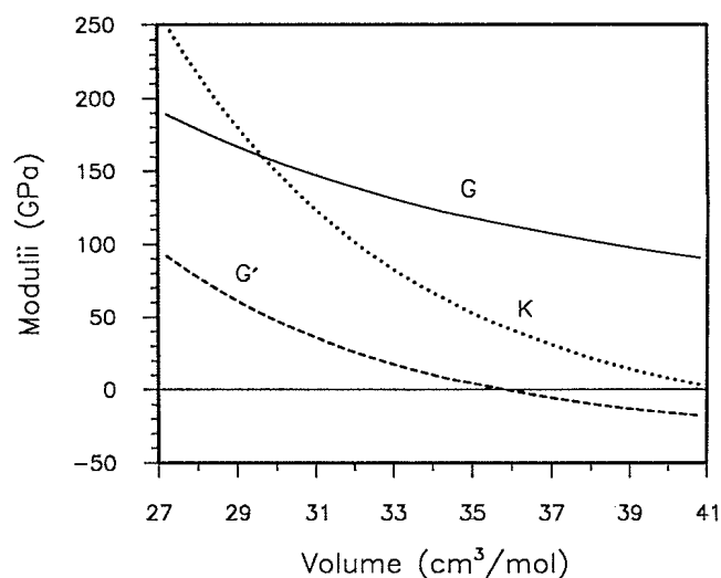
FIG. 4. Evaluation of the Born stability criteria for \text{CaSiO}_3 perovskite as a function of volume derived from the lattice-dynamical calculations. The first mechanical instability in the Pm\bar{3}m structure occurs for G' at 36 cm 3 /mol followed by an instability in K at 41 cm 3 /mol. Note that all of the generalized moduli are positive at 31 cm 3 /mol, the onset of structural disordering observed in the constant volume MD simulations.
