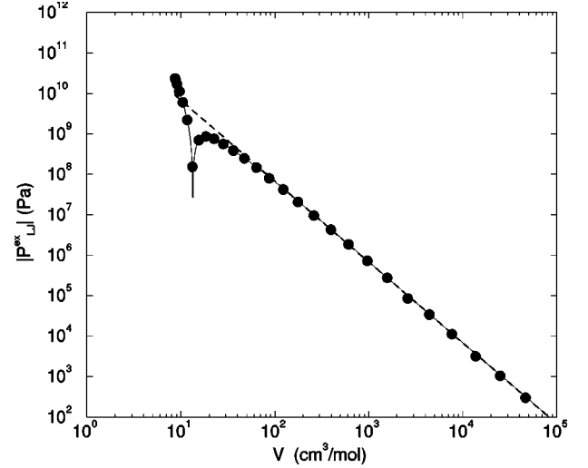
FIG. 5. Isotherm of |P_{LJ}^{ex}| for the LJ fluid at T=4000 K. The solid line is the fit to Eq. (23) with M=8 . The dashed line is the curve given by Eq. (20). The data are shown on a log-log plot to simplify the comparison of the data to Eq. (20) at large V . The cusp near V=10 cm 3 /mol is due to the fact that P_{LJ}^{ex} changes sign.
