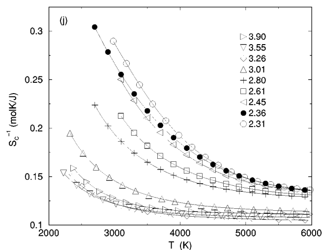
FIG. 14. (a)–(i) S_c along isochores; each panel is labeled by the density in \text{g}/\text{cm}^3 . Each curve is obtained using Eq. (9), by integrating the fitted curves for e_{1S} shown in Fig. 12. Dotted curves are fits to a two-state model [43,44]. (j) 1/S_c as a function of T .
