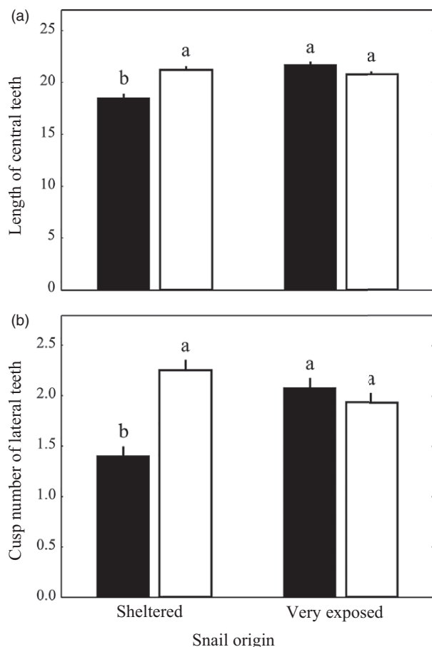
Fig. 4. (a) Length of central teeth (in \mu\text{m} ) and (b) number of cusps in lateral teeth (mean \pm SE) of radulae in Littorina obtusata fed Fucus vesiculosus from sheltered (black bars) or exposed (white bars) habitats in Nova Scotia. Treatments sharing the same letter did not differ significantly from one another.
