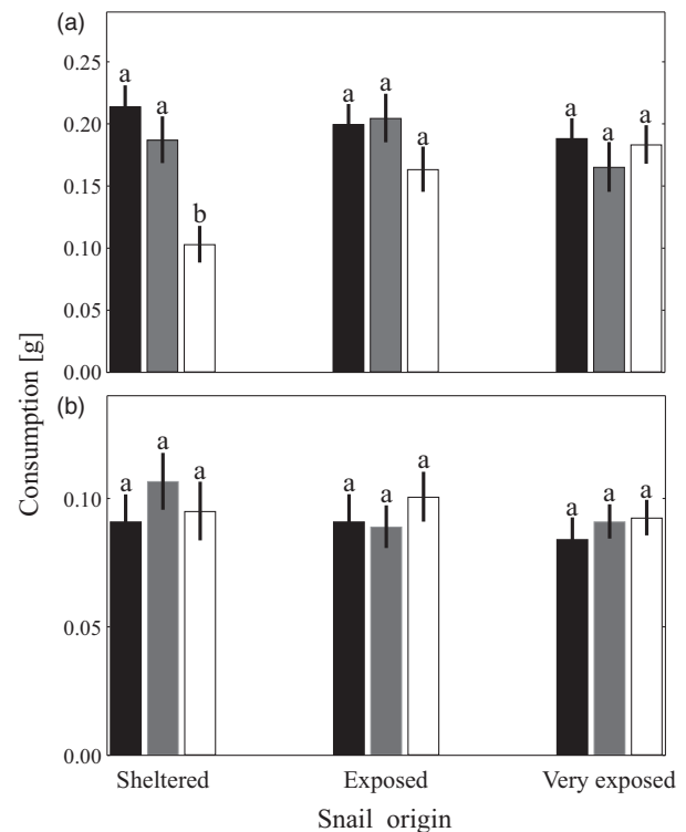
Fig. 3. Littorina obtusata consumption (mean \pm SE) of (a) live Fucus vesiculosus fragments and (b) reconstituted food made of F. vesiculosus from a sheltered (black bars), exposed (dark grey bars) and very exposed (white bars) site in Nova Scotia. Treatments sharing the same letter did not differ significantly from one another.
