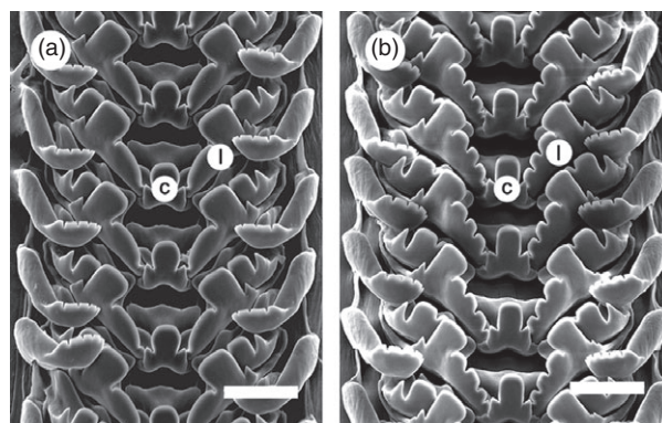
Fig. 1. Thirty degree-tilted top view of the radula of Littorina obtusata from (a) sheltered and (b) exposed habitats in Nova Scotia, showing (c) central (rachidian) and (l) lateral teeth. Scale bar = 50 µm.
