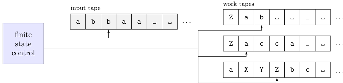
Figure 1: An illustration of a k -tape Turing machine.
